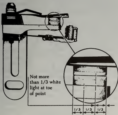
FIGURE 4-67. Checking breaker contact area.
